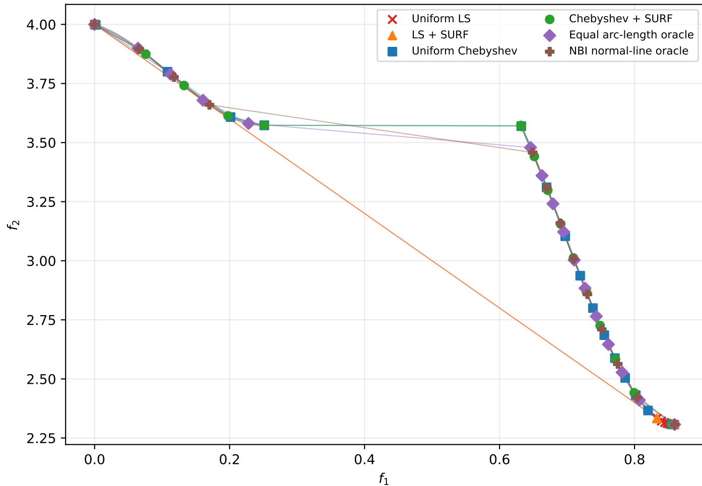
DTLZ7 (M=2): deterministic front-oracle diagnostic
